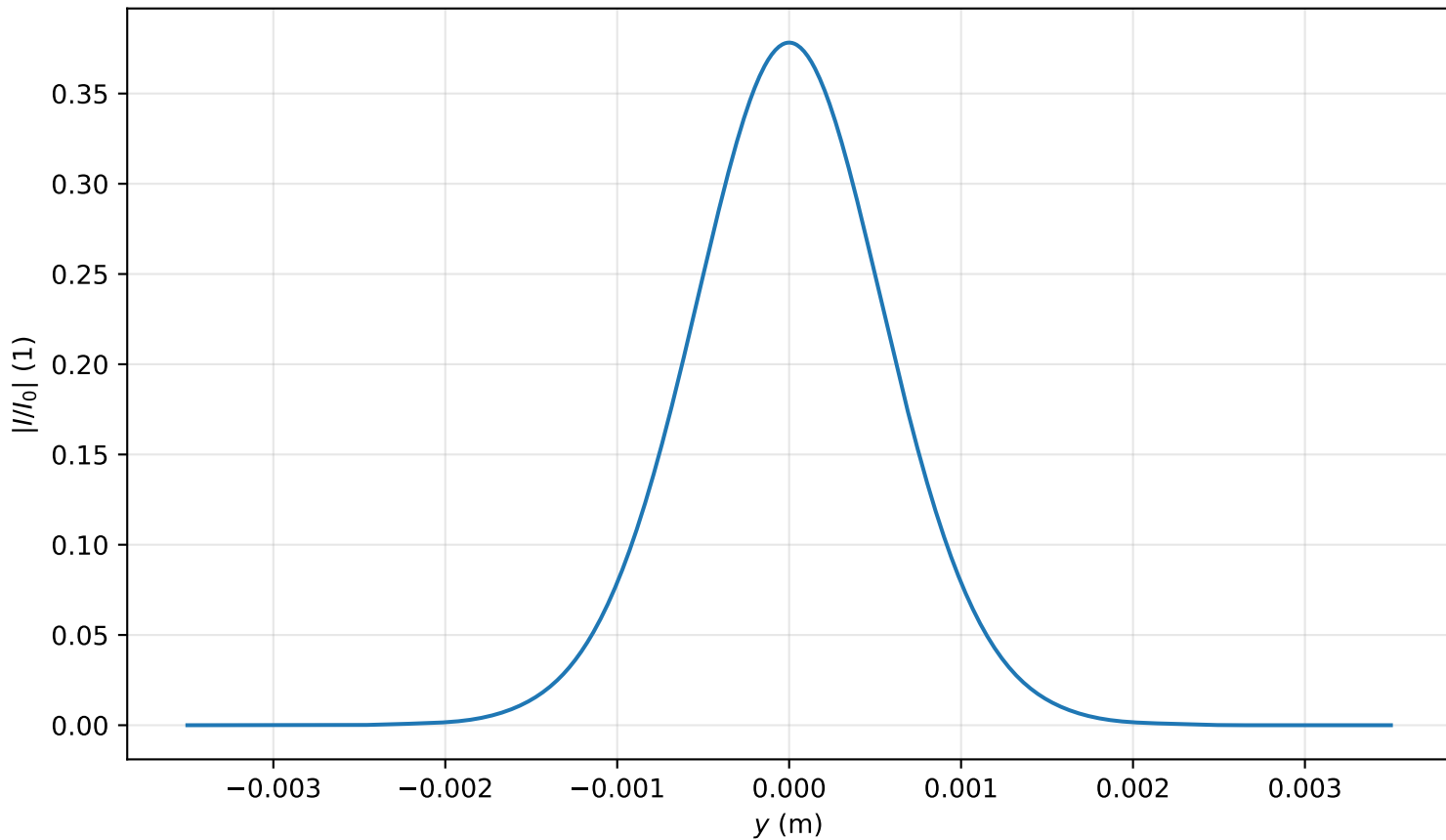
Intensity profile I(x=0, y, z=3.264)/I_0 , P_{in}=0.3P_{cr} , artificial time
